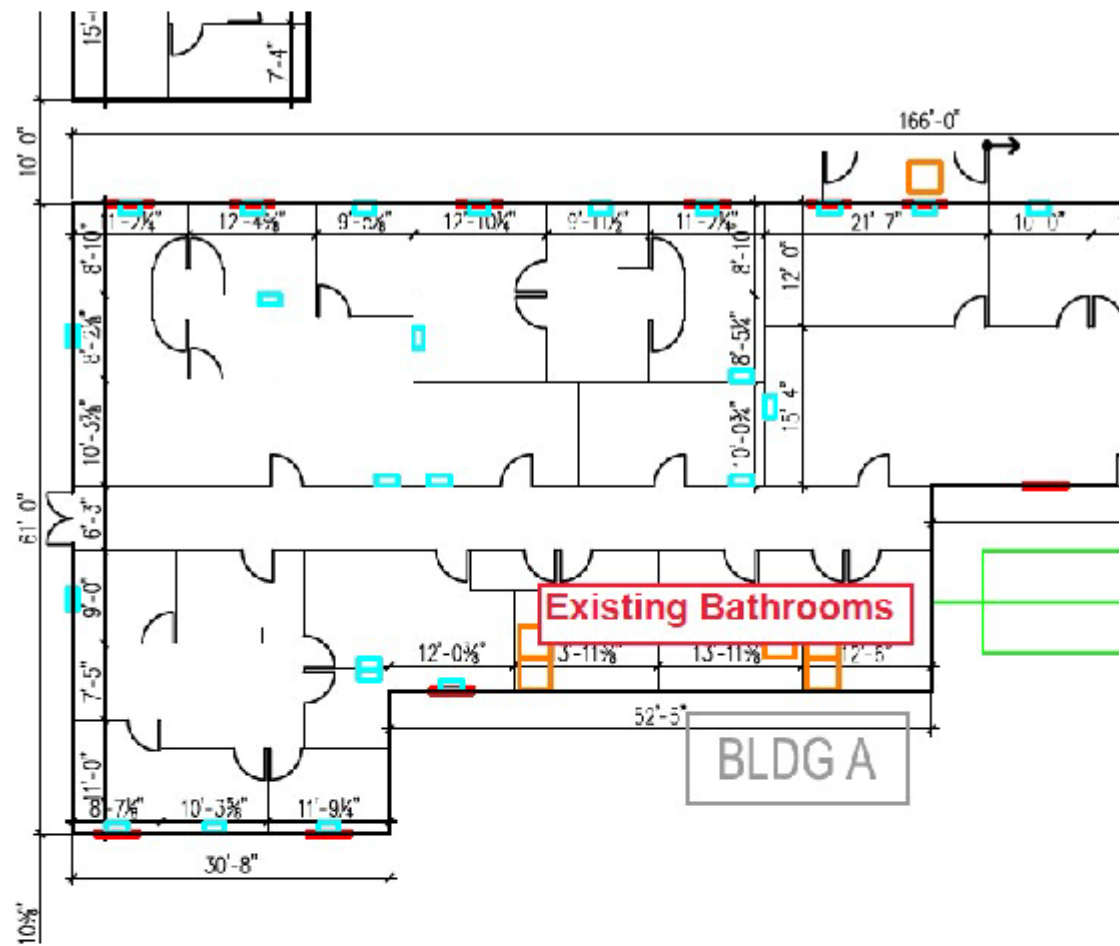
Attachment A- Existing Floor Plan_ Partial
